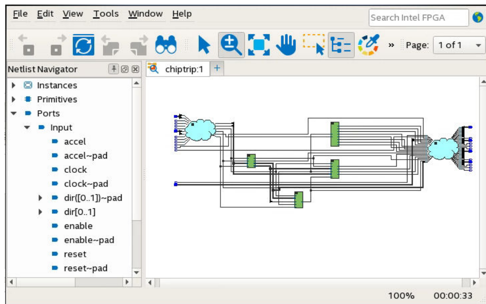
Figure 103. Technology Map Viewer
