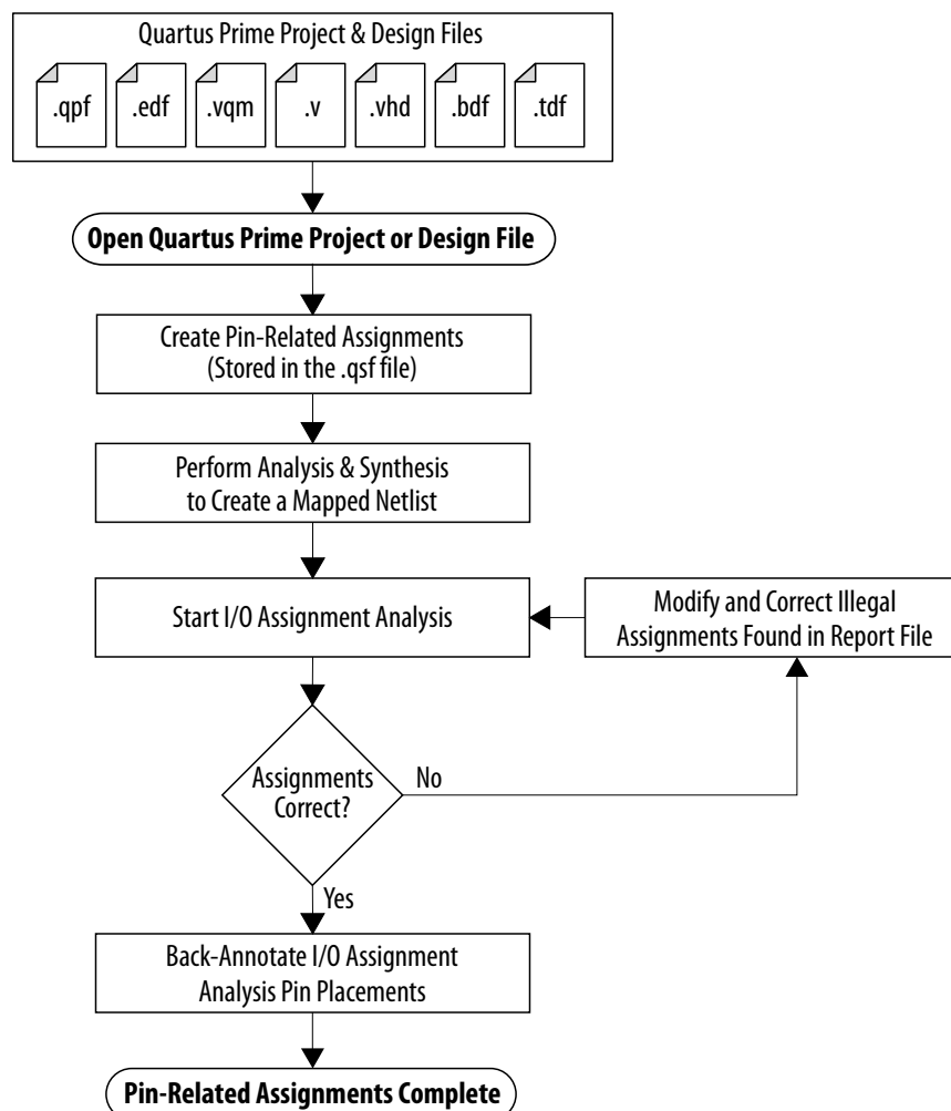
Figure 74. I/O Assignment Analysis Flow
