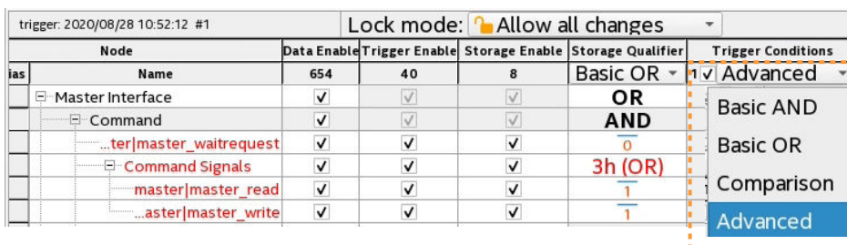
Figure 43. Accessing the Advanced Trigger Condition Tab
