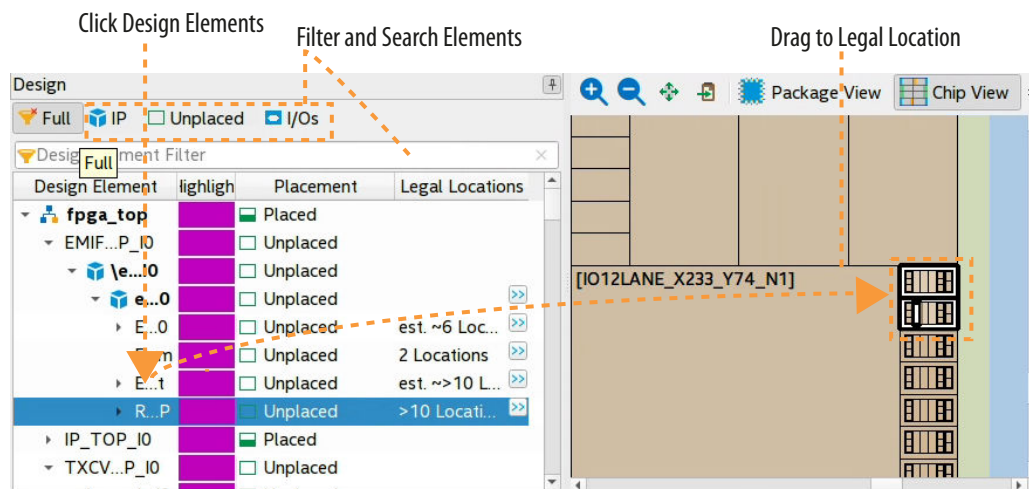
Figure 14. Interface Planner (Plan Tab)
