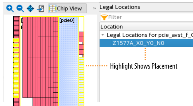
Figure 43. IP Placed In Legal Tile Location
