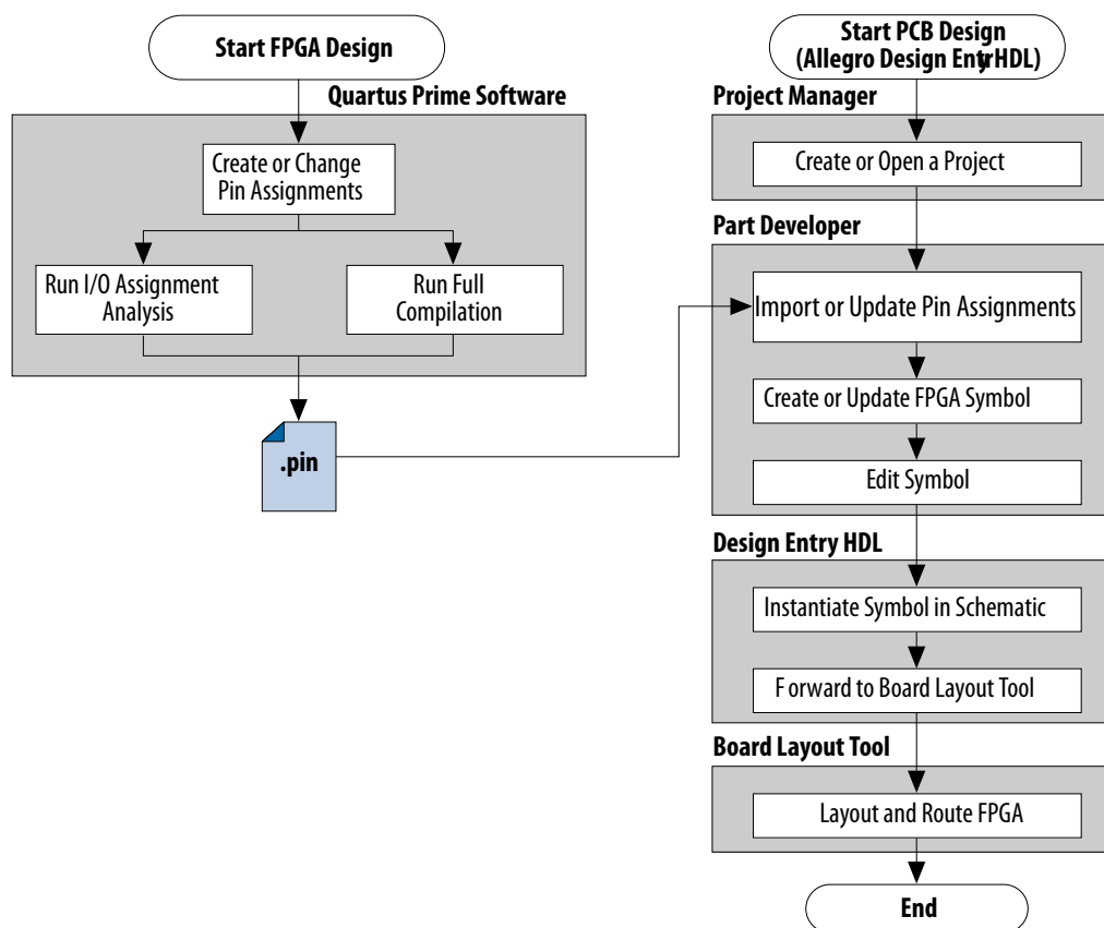
Figure 20. Design Flow with the Cadence Allegro Design Entry HDL Software
