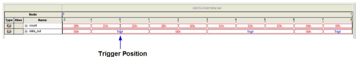
Figure 86. Signal Tap Logic Analyzer Conditional Data Capture
