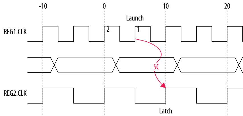
Figure 139. Default Setup Check Analysis
