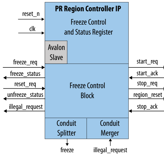
Figure 73. Partial Reconfiguration Region Controller IP Core
