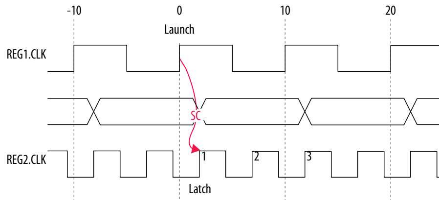
Figure 133. Setup Timing Diagram
